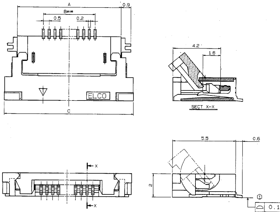
Figure 31: Mechanical dimensions of ZIF connector
