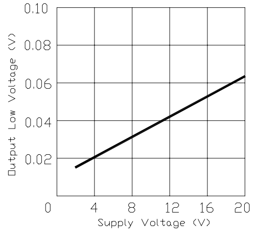
Fig. 2 Output Low Voltage V.S. Supply Voltage
