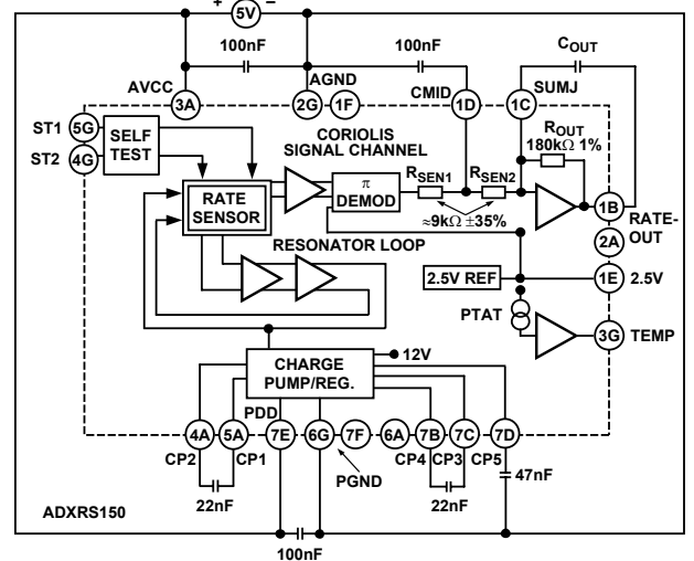
Figure 23. Block Diagram with External Components
