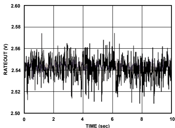
Figure 24. Random Vibration (Lateral) 10 kHz to 20 kHz at 0.01 \text{ g}/\sqrt{\text{Hz}} with 60 Hz Sampling and 0.5 sec Averaging
