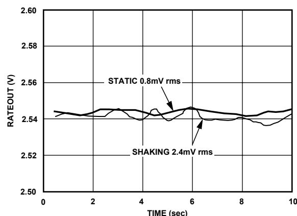
Figure 26. Random Vibration (Lateral) 10 kHz to 20 kHz at 0.01 \text{ g}/\sqrt{\text{Hz}} with 60 Hz Sampling and 0.5 sec Averaging
