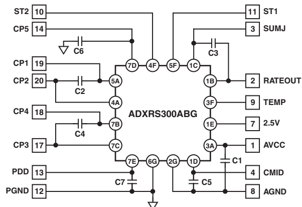
Figure 1. ADXRS300EB Schematic
