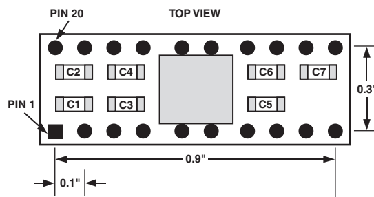
Figure 2. ADXRS300EB Parts Layout
