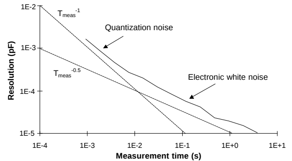
Figure 3 The resolution after the calculation required for the three-signal technique versus the total measurement time. The measurement range equals 0 - 2 pF and C_p = 50 pF (see Figure 7).
