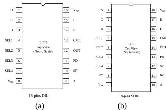
Figure 1 Pin configuration.
