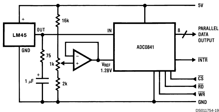
FIGURE 12. Temperature To Digital Converter (Parallel TRI-STATE® Outputs for Standard Data Bus to \mu P Interface) (128°C Full Scale)
