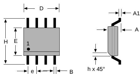
HMC1021S—8-Pin SOIC
